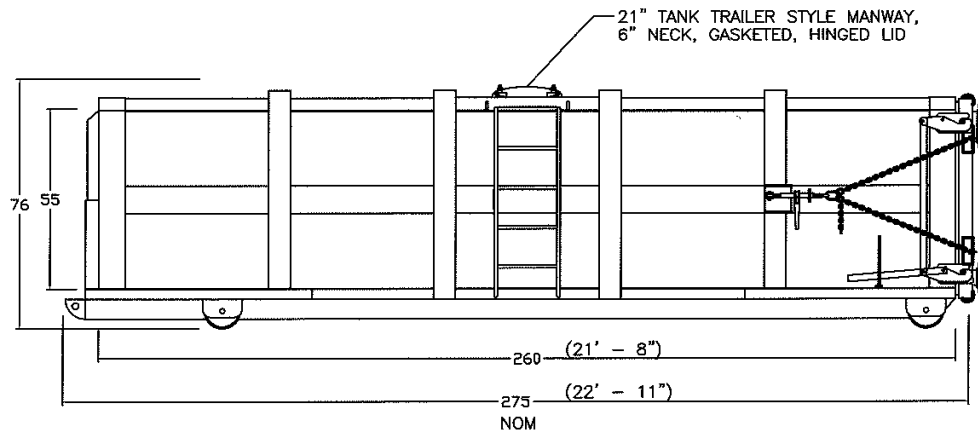
HEAVY DUTY DRAGON VACUUM LOAD CONTAINER
