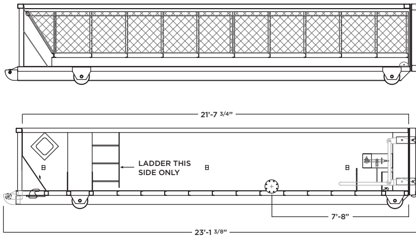
Side View
